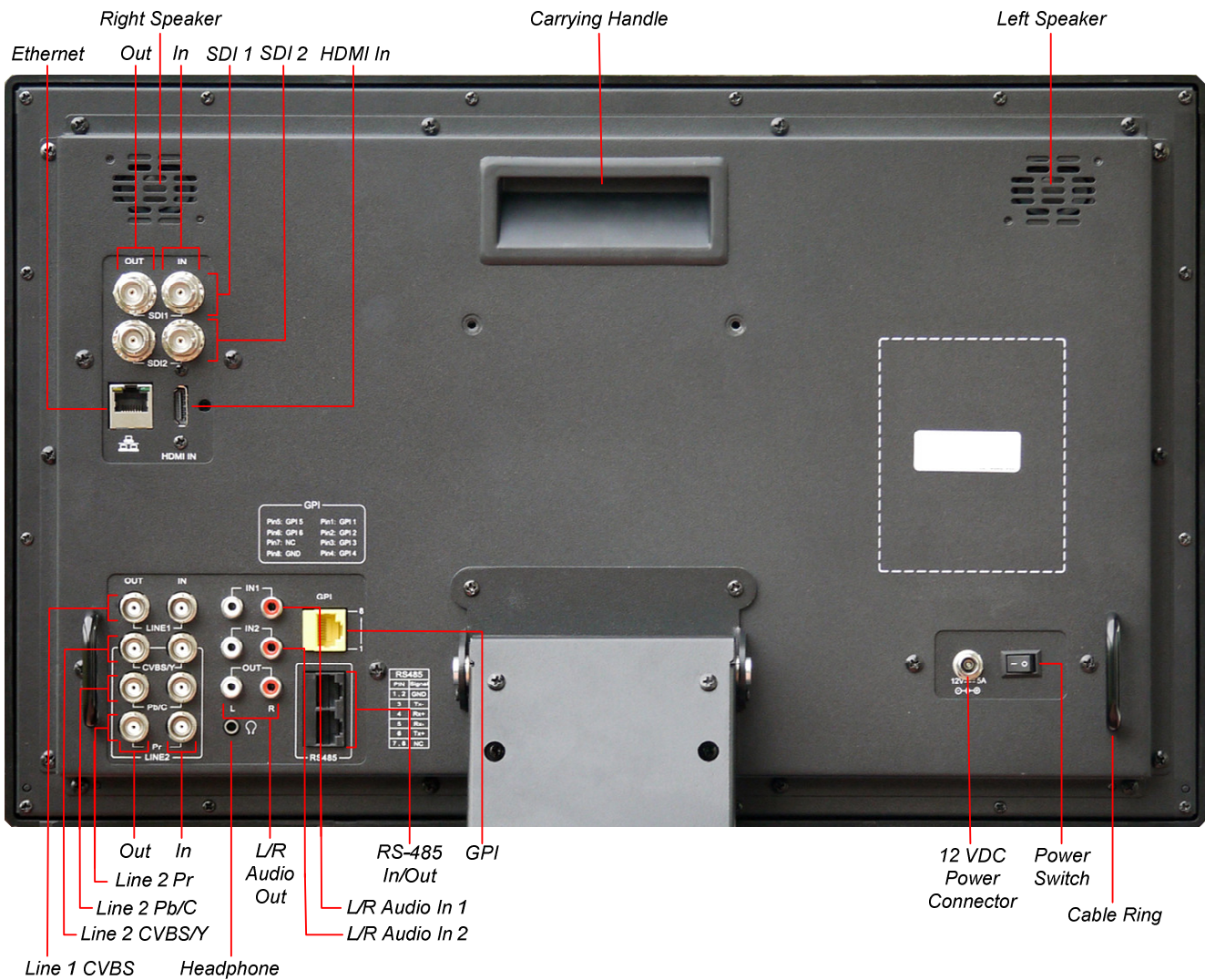
Figure 2-3: RMT-173-3G Series Rear Panel Layout
