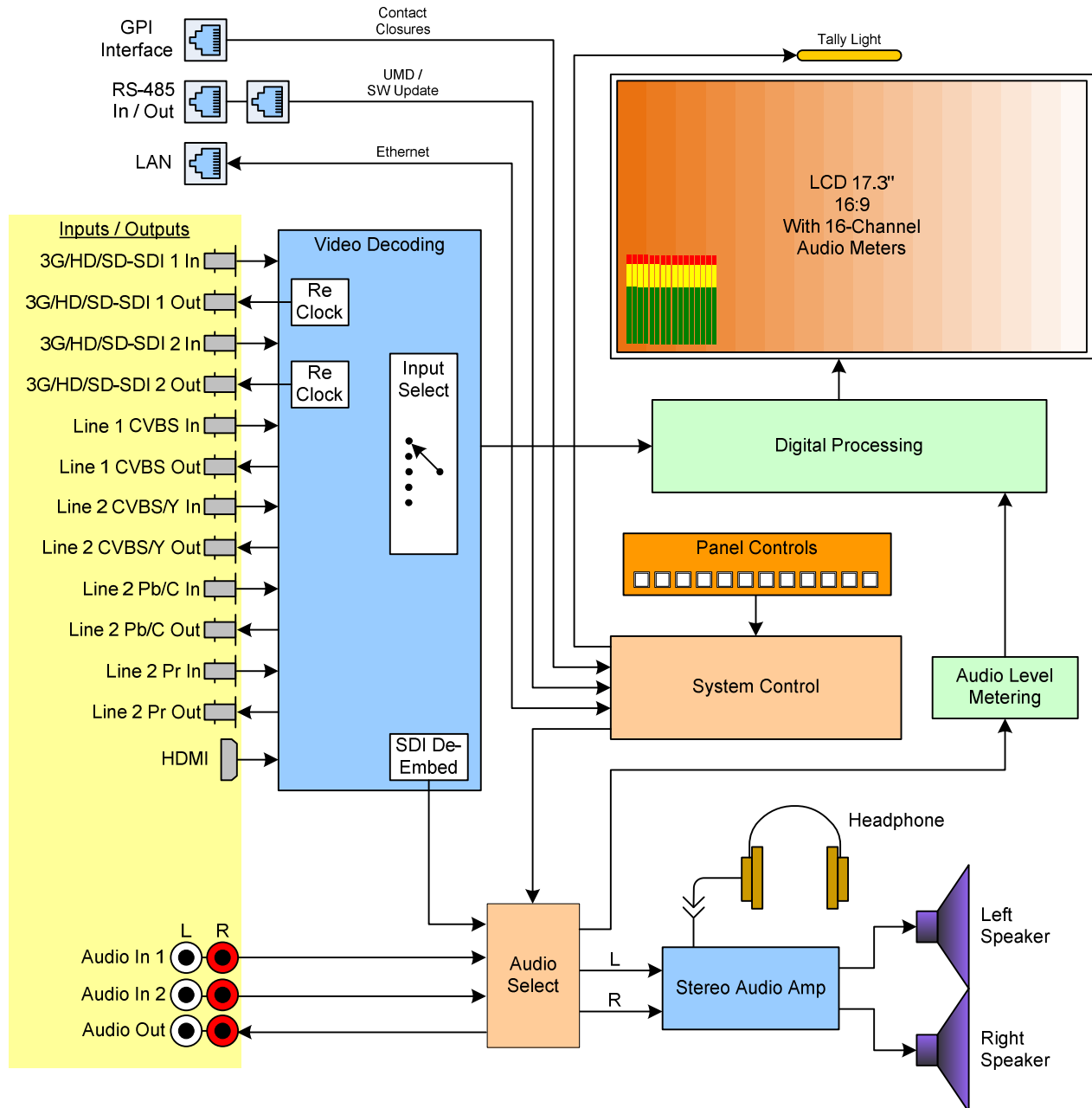
Figure 3-1: RMT-173-3G Series Block Diagram
