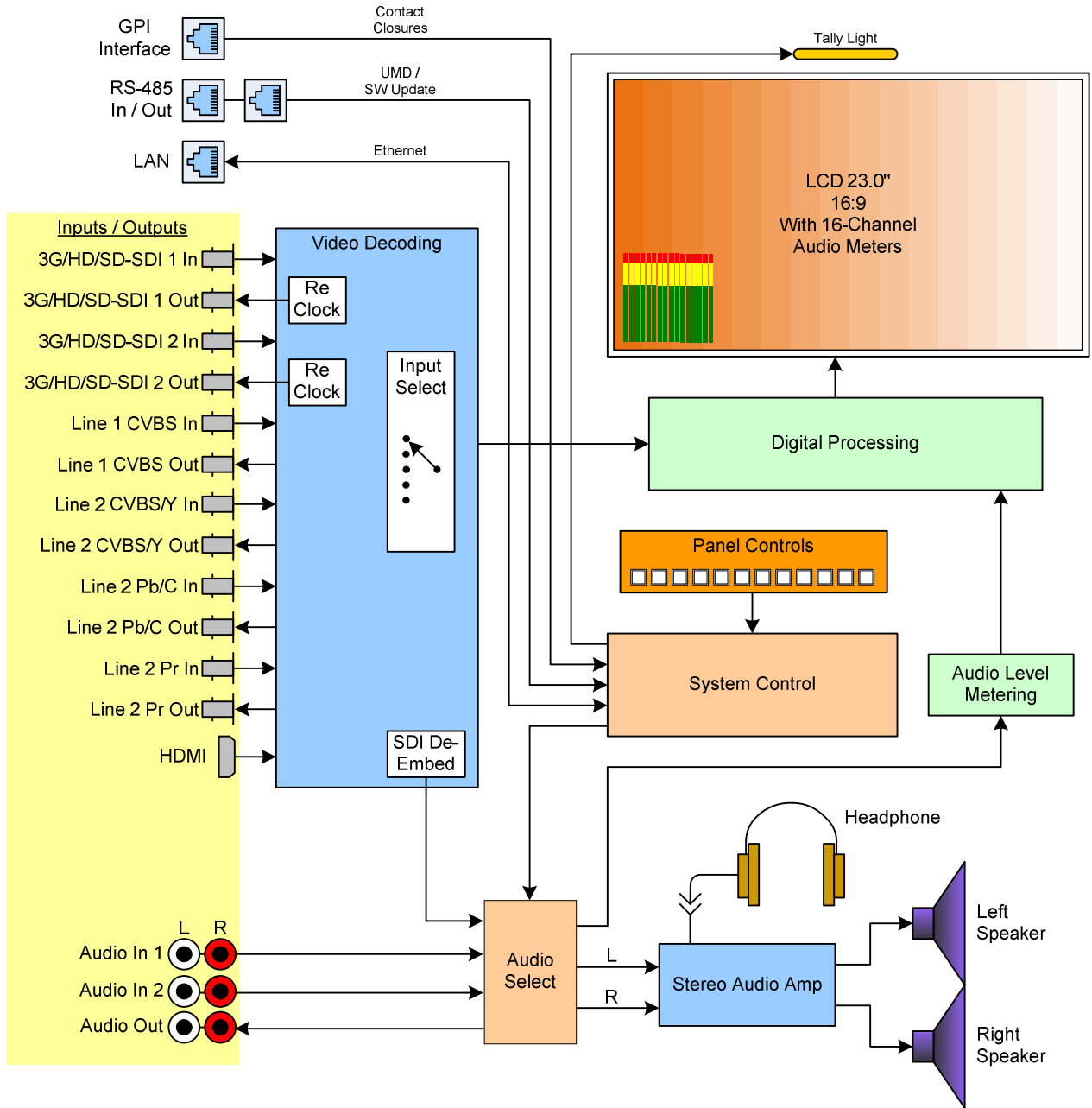
Figure 3-1: RMT-230-3G Block Diagram
