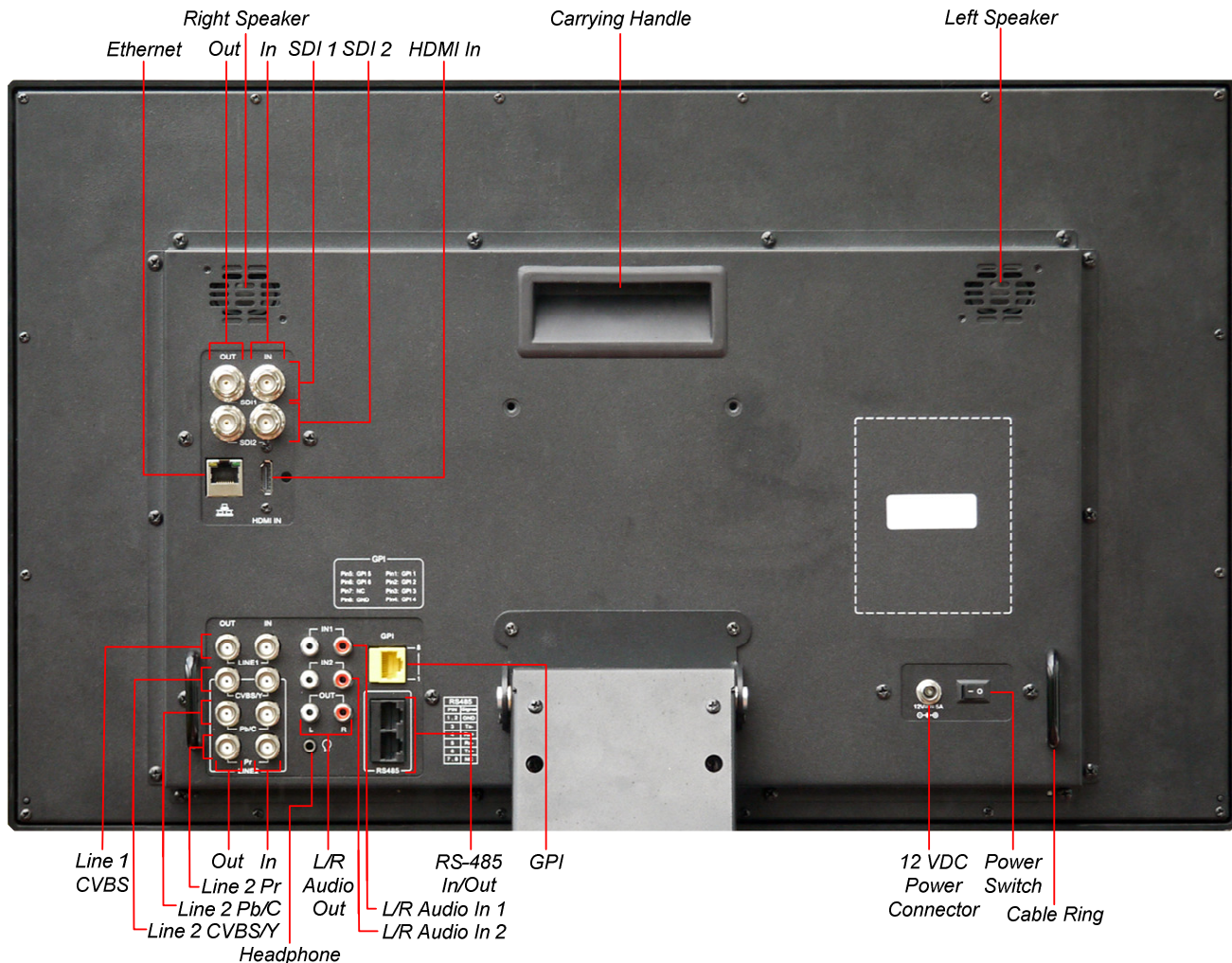
Figure 2-3: RMT-230-3G Rear Panel Layout
