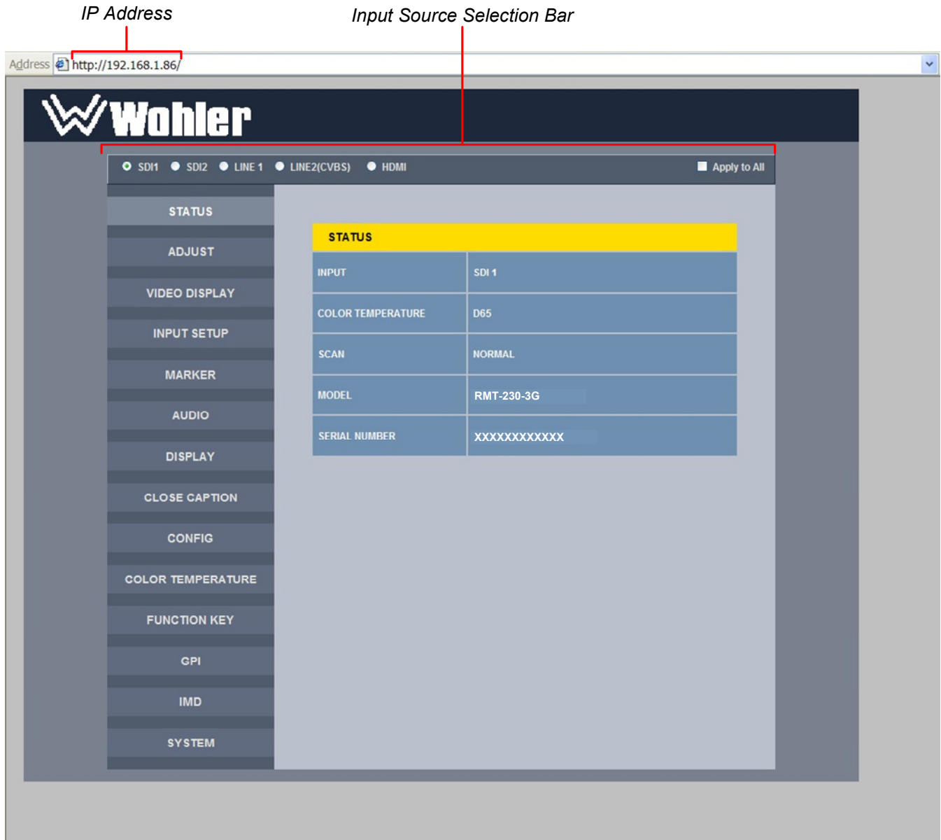
Figure 4-2: Status Page
