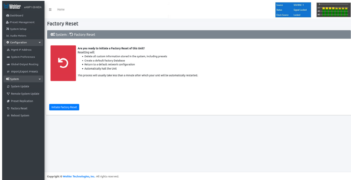
Figure 4–25: Factory Reset
