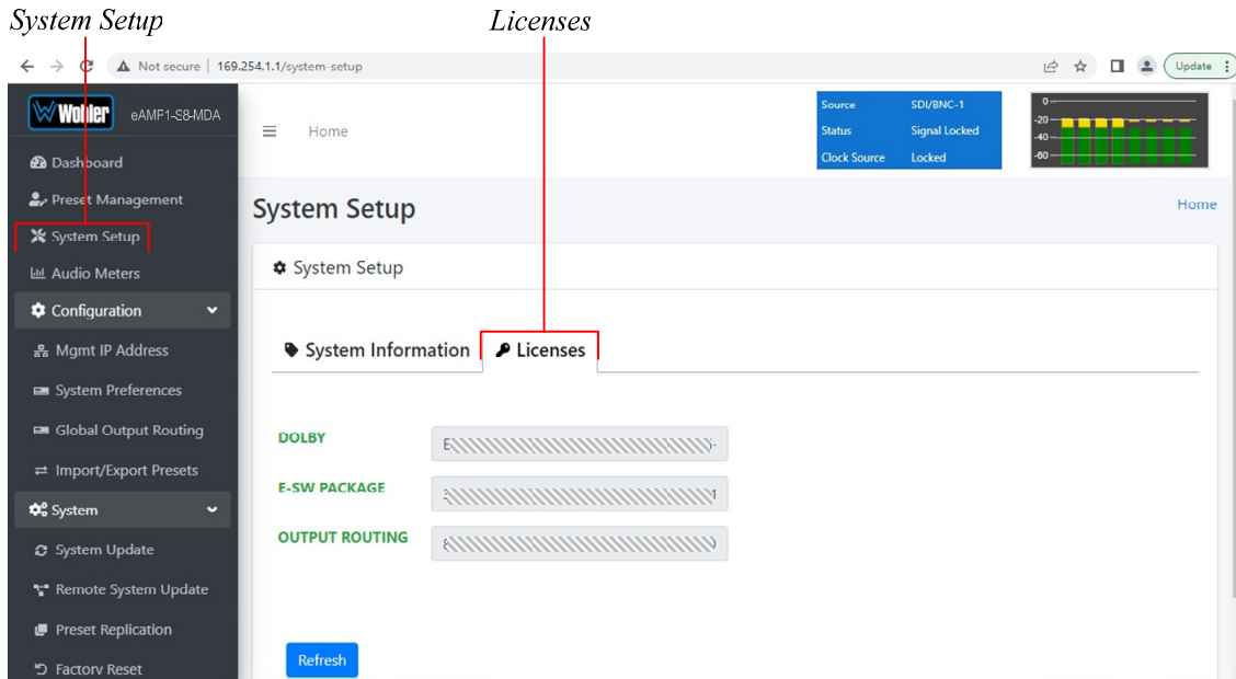
Figure 4-24: Licenses Tab
