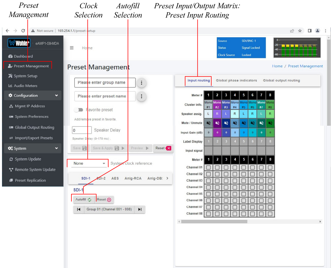
Figure 4–15: Configure Presets
