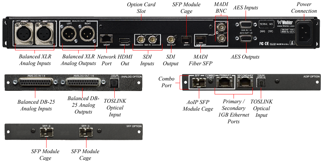
Figure 2-2: iVAM1-SUM Rear Panel & Option Cards
